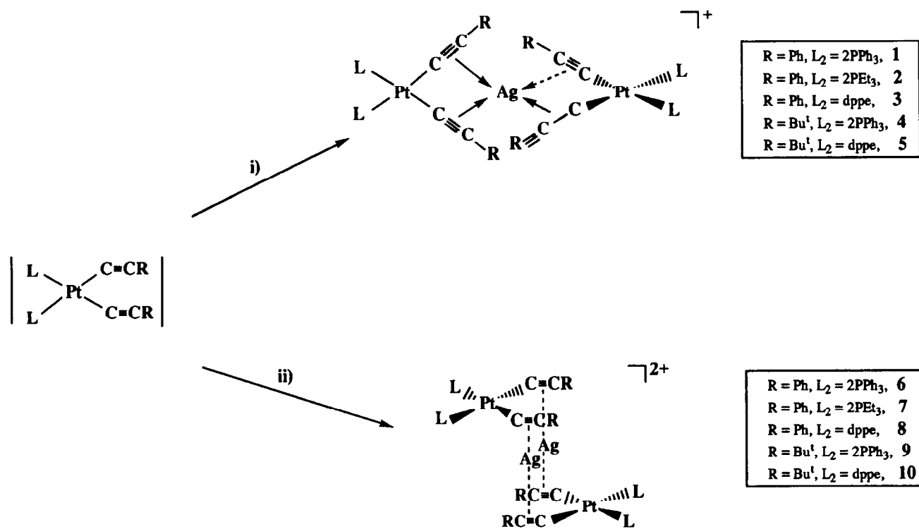
Scheme 1. (i) 0.5 equivalents of \text{AgClO}_4 in acetone; (ii) 1 equivalent of \text{AgClO}_4 in acetone.
